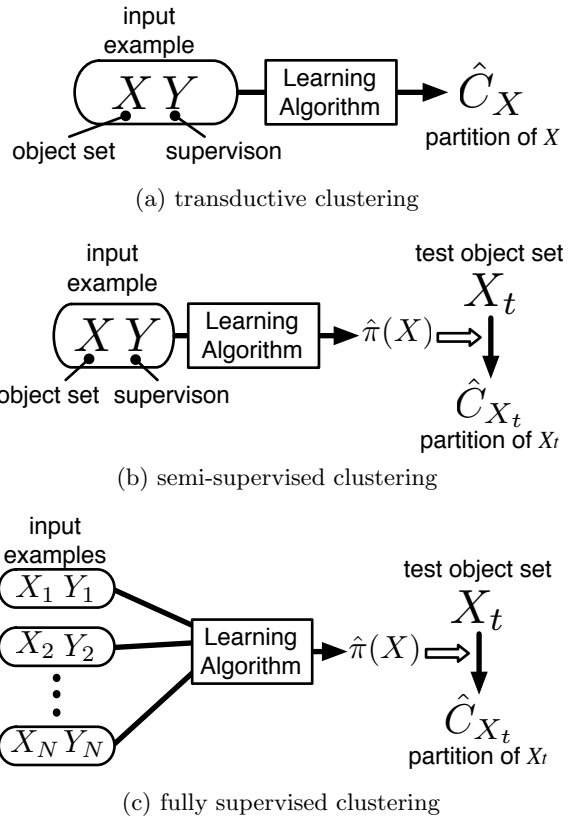
Figure 1: Three types of supervised clustering problems
