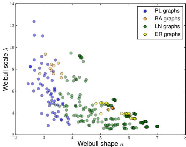
Figure 3: Two-dimensional embedding of shortest path histograms obtained for different kinds of graph topologies. Each point (\kappa, \lambda) represents a path length distribution in terms of the parameters of the best fitting Weibull model. Path length distributions obtained from different types of graphs appear to confined to specific regions.
