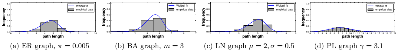
Figure 1: Examples of Weibull fits to the shortest path length distributions of an ER, a BA, an LN, and a PL graph. The empirical distributions are either skewed to the left or more or less symmetric; the Weibull mimics this behavior well and closely models the histograms.
