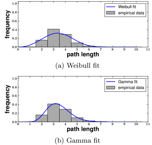
Figure 2: Example of a Weibull and a Gamma fit to the shortest path length distribution of a PL graph ( \gamma = 2.3 ). The empirical distribution is noticeably skewed to the right and the Gamma distribution provides the better model.
