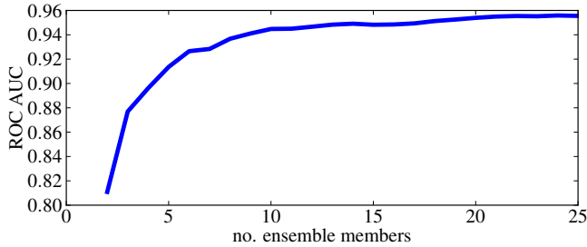
Figure 3: Quality with increasing ensemble size.
