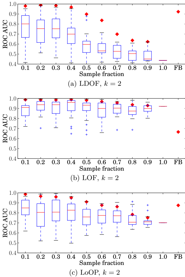
Figure 5: ROC AUC for ensemble members of the subsampling ensemble for different sample sizes (boxes), the base method (sample size=1.0), and ensembles (diamonds)—on top of subsamples and feature bags (FB)—on dataset Lymphography.
