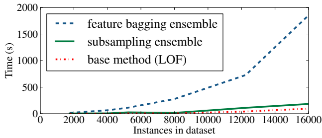
Figure 2: Runtime of LOF, subsampling ensemble, and feature bagging when increasing database size.
