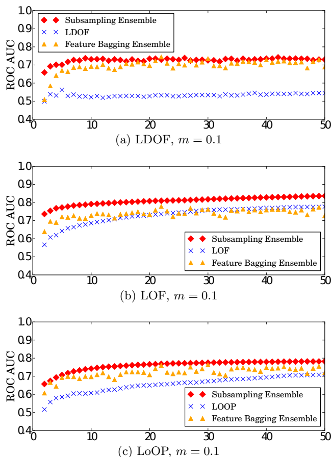
Figure 8: ROC AUC for base methods and corresponding ensembles varying k on dataset waveform.
